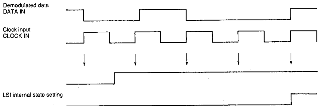
Pin Read-In Timing during Synchronization Detection
