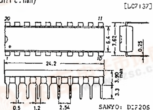
Case Outline 3008A-D201C (unit:mm)
