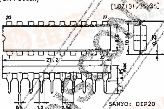
Case Outline 3021B-D20S1C (unit:mm)
