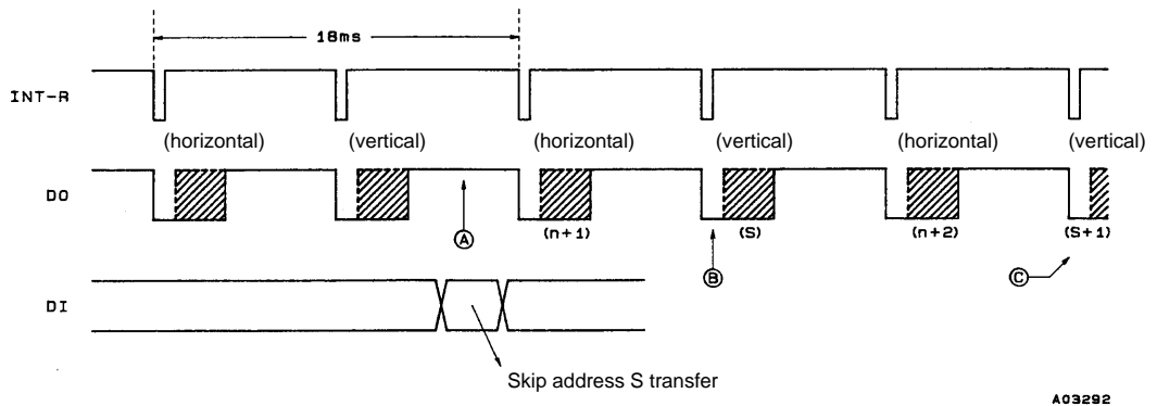
Figure 5 Address Skip
