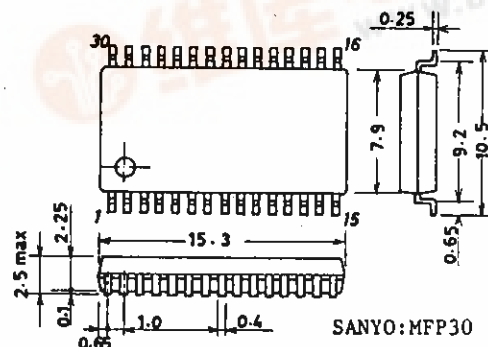
Package Dimensions 3073A [LC7367JM] (unit : mm)
