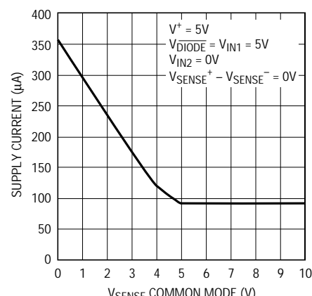
DC Supply Current vs V_{\text{SENSE}}
