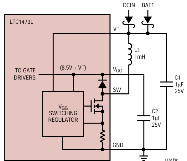
Figure 1. V_{GG} Switching Regulator
