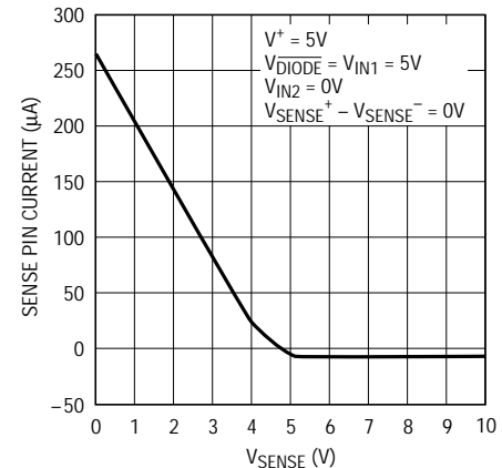
SENSE Pin Source Current ( I_{\text{SENSE}} ) vs V_{\text{SENSE}}
