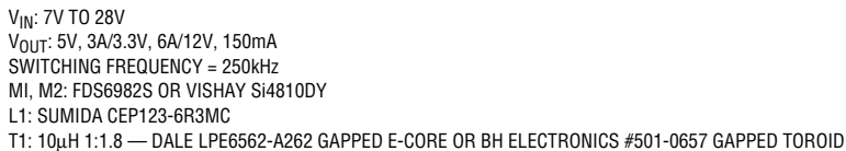
Figure 12. LTC3728L/LTC3728LX High Efficiency Low Noise 5V/3A, 3.3V/5A, 12V/120mA Regulator
