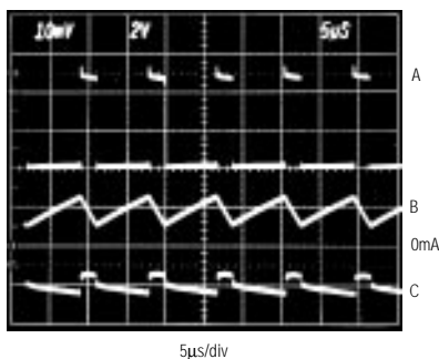
SWITCHING WAVEFORMS, CONTINUOUS CONDUCTION
