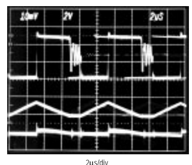
SWITCHING WAVEFORMS, DISCONTINUOUS CONDUCTION
