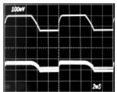
LINE-TRANSIENT RESPONSE
