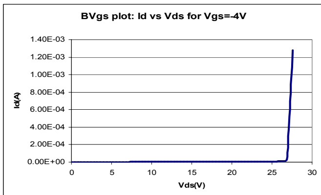
Figure 3 – Breakdown Voltage V_{ds} vs I_d
