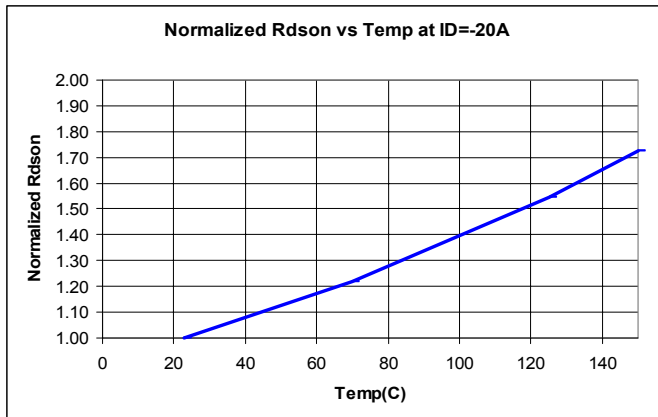
Figure 7 – R_{\text{DS(on)}} Temperature Coefficient
