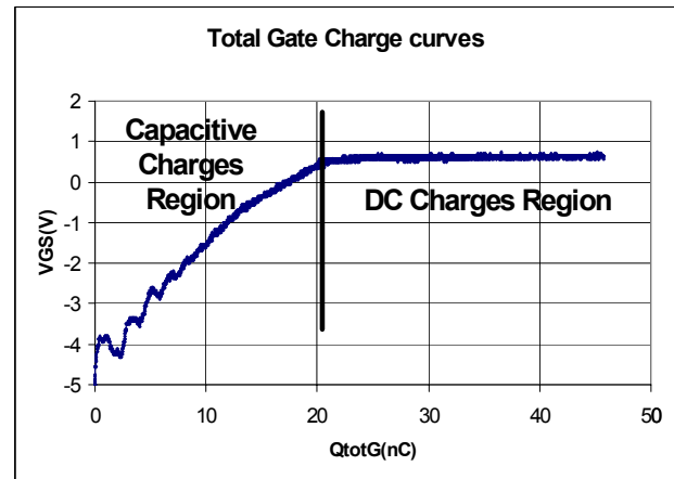
Figure 2 – Total Gate Charge
