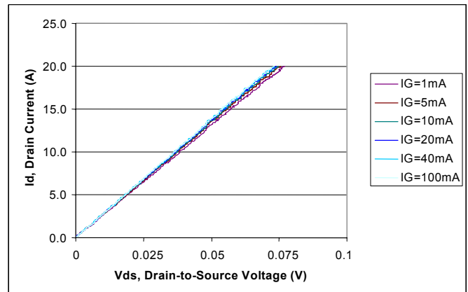
Figure 8 – On-Region Characteristics
