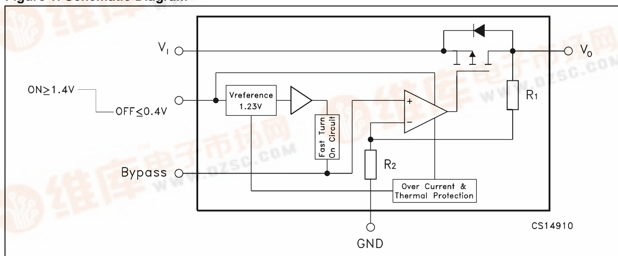
Figure 1: Schematic Diagram
