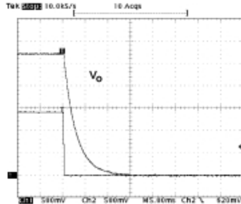
Figure 22: TURN-OFF
