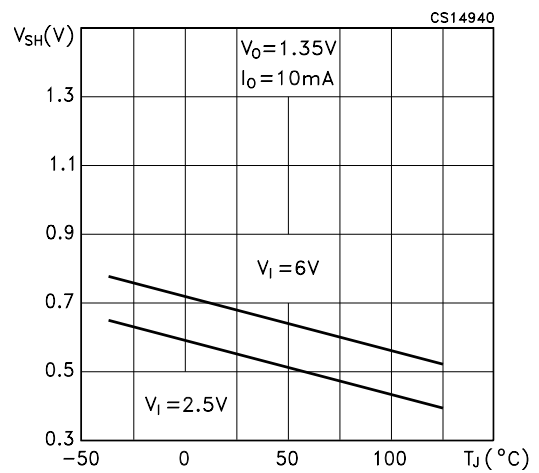
Figure 7: Shutdown Voltage vs Temperature
