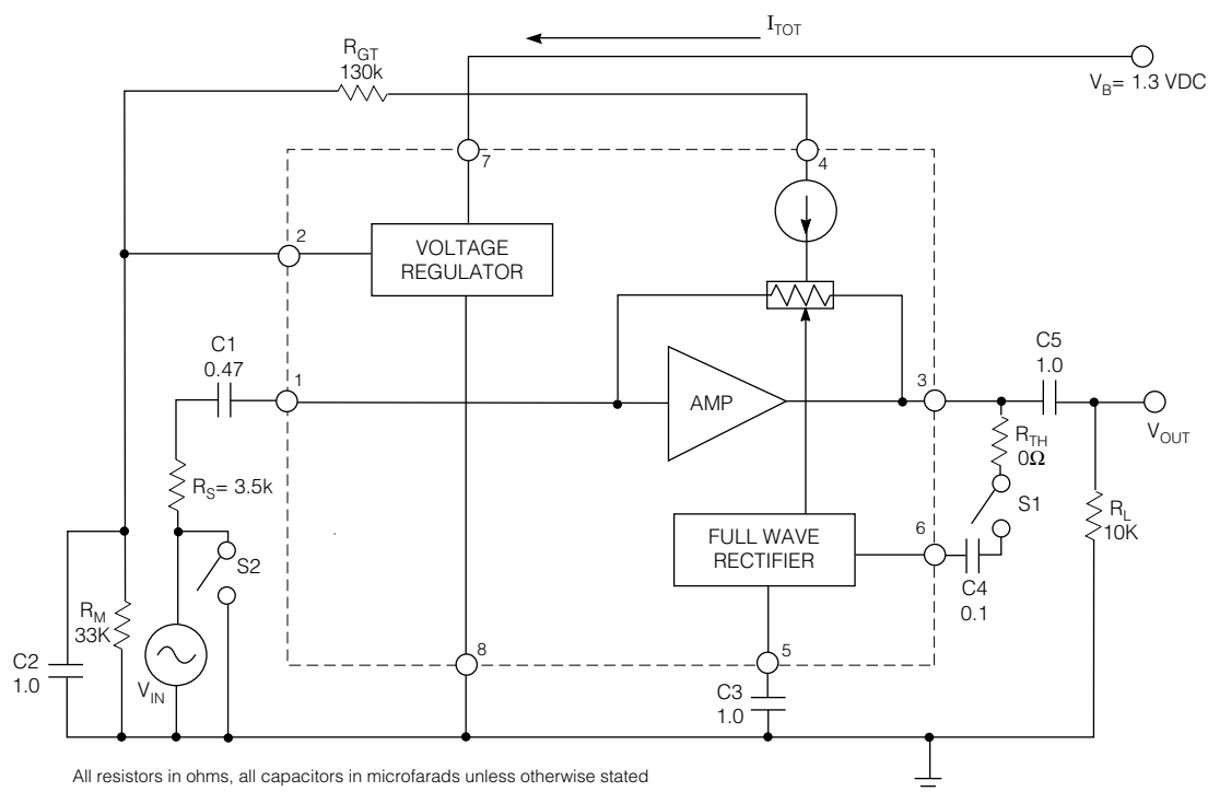
Fig. 1 Test Circuit
