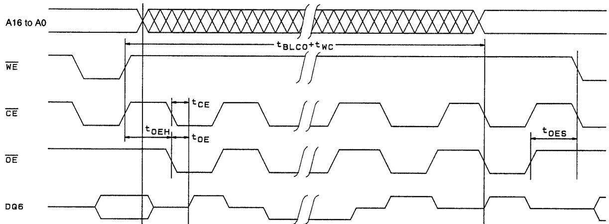
Figure 5 Toggle Bit
