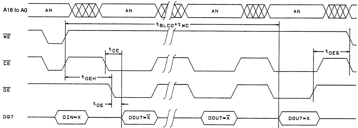
Figure 4 Data Polling
