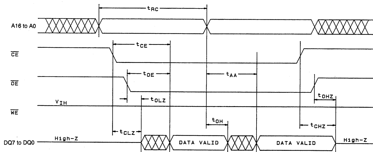
Figure 1 Read Cycle
