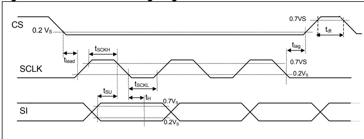
Figure 7: Input Timing Diagram
