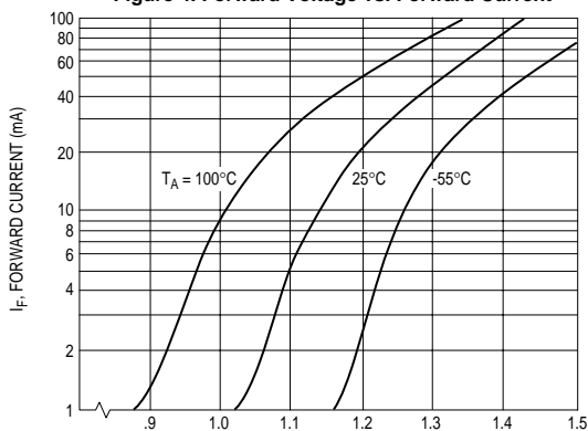
Figure 4. Forward Voltage vs. Forward Current
