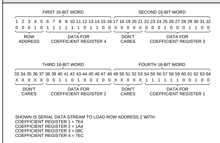
FIGURE 2. SERIAL DATA FORMAT
