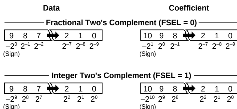
FIGURE 1A. INPUT FORMATS
