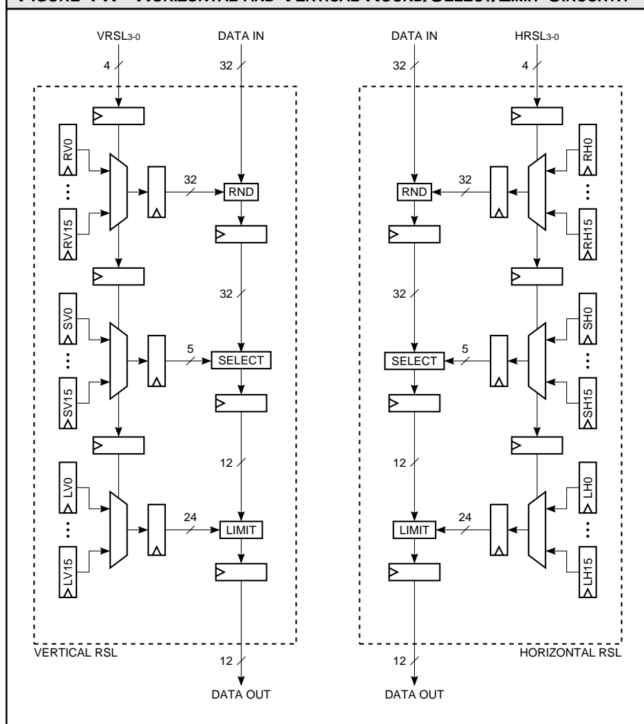
FIGURE 11. HORIZONTAL AND VERTICAL ROUND/SELECT/LIMIT CIRCUITRY
