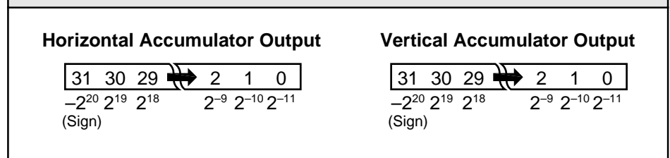
FIGURE 3. HORIZONTAL AND VERTICAL ACCUMULATOR FORMATS
