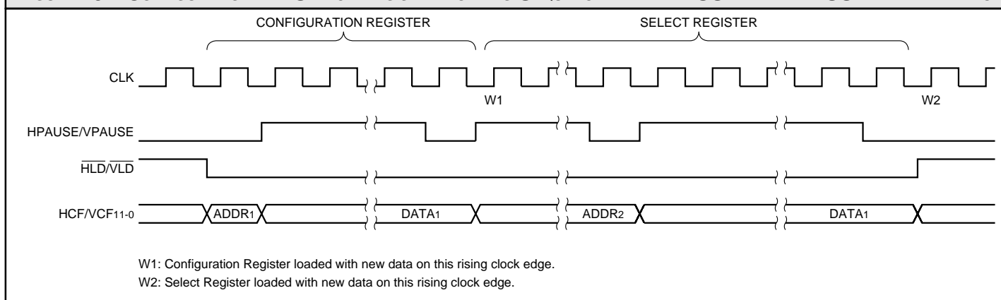
FIGURE 15. CONFIGURATION AND SELECT REGISTER LOADING SEQUENCE WITH HPAUSE AND VPAUSE IMPLEMENTATION
