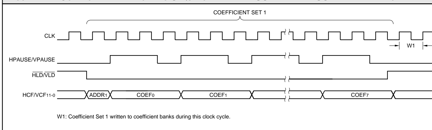
FIGURE 14. COEFFICIENT BANK LOADING SEQUENCE WITH HPAUSE AND VPAUSE IMPLEMENTATION
