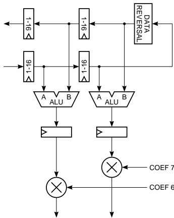
EVEN-TAP MODE
