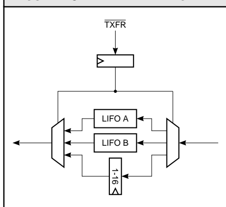
FIGURE 10. DATA REVERSAL
