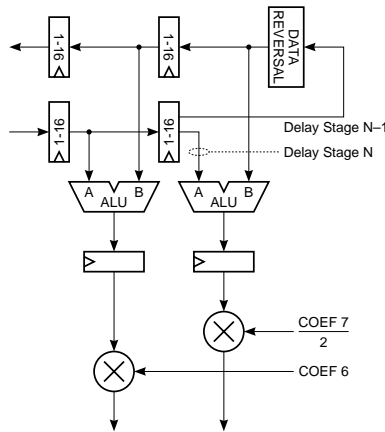
ODD-TAP MODE
