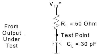
Figure 1. Load Circuit [15]
