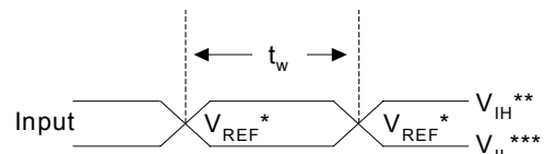
Figure 5. Voltage Waveforms Pulse Duration [18,19]
