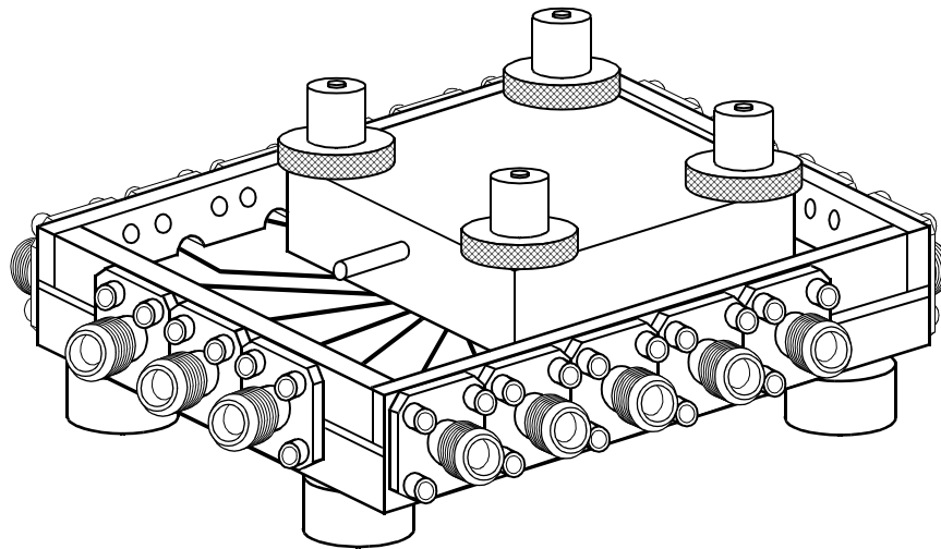
Figure 15. TF1004A Test Fixture
