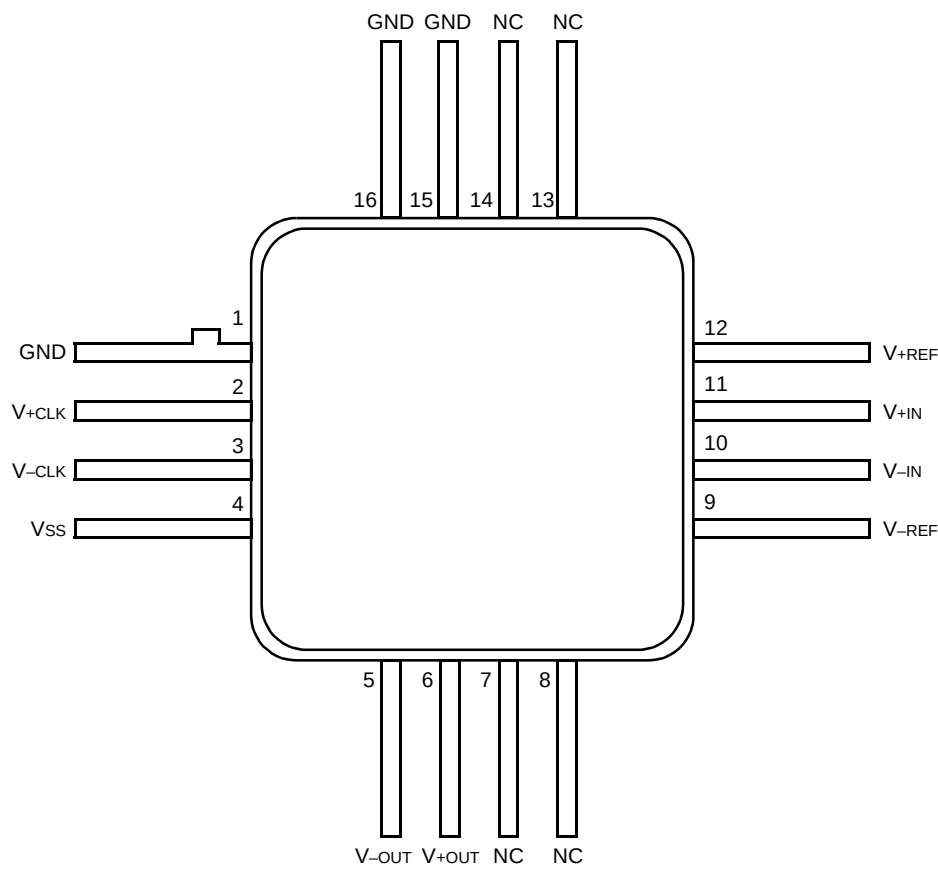
Figure 2. Pin Diagram
