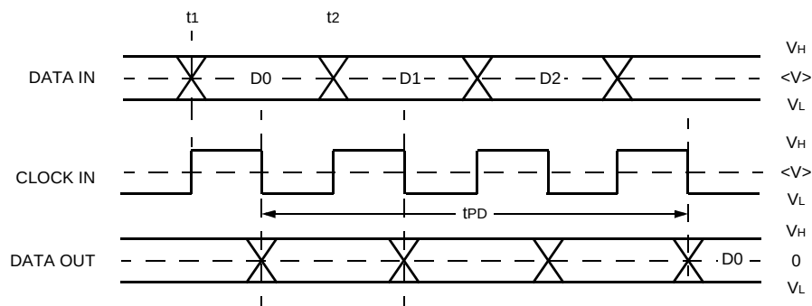
Figure 3. Timing Diagram
