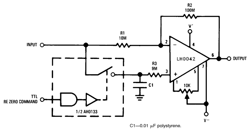
Re-Zeroing Amplifier
