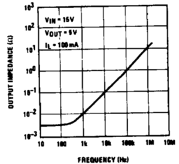
Output Impedance
