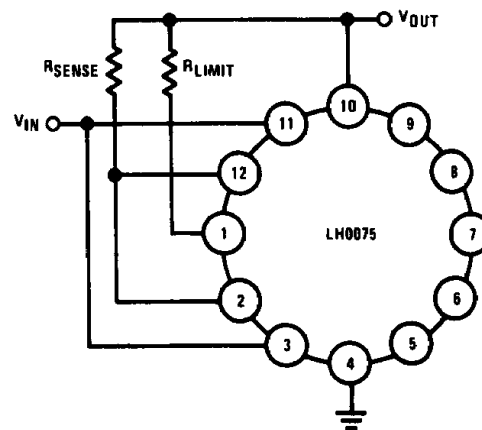
TL/H/5549-5
