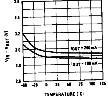
Input-Output Differential Voltage
