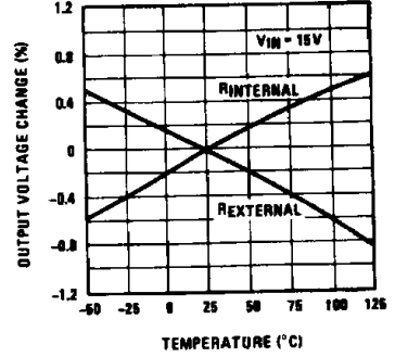
Temperature Stability
