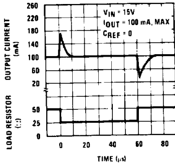
Load Transient Response (Current Mode)
