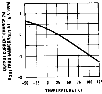
Current Limit
