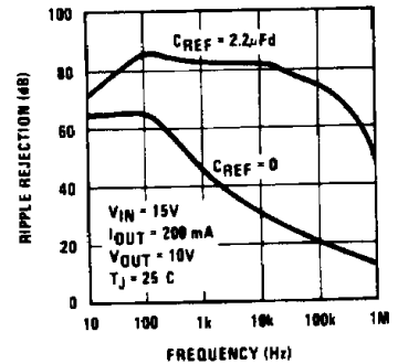
Ripple Rejection
