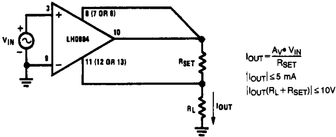
FIGURE 13. Output Current Source Connection
