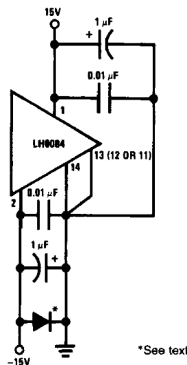
FIGURE 5. Power Supply Connections
