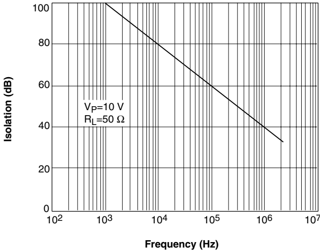
Figure 9. Output Isolation
