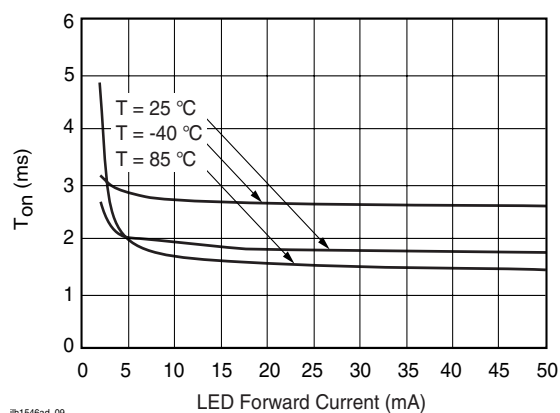
Fig. 9 Turn-on Time vs. LED Current
