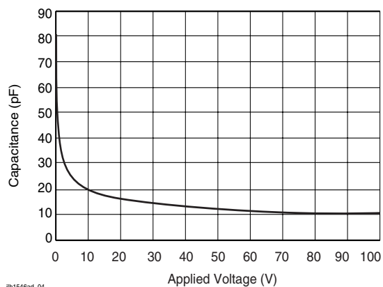
Fig. 5 Switch Capacitance vs. Applied Voltage
