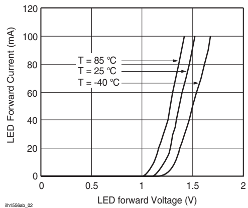
Figure 3. LED Forward Current vs. LED Forward Voltage
