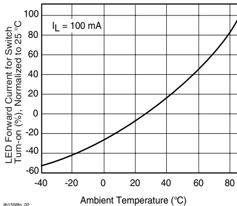
Figure 2. LED Current for Switch Turn-on vs. Temperature
