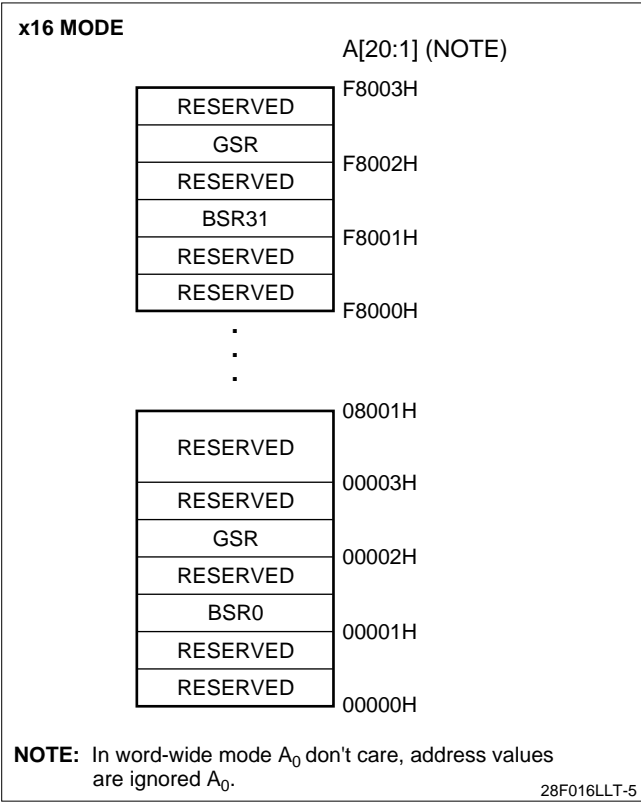
Figure 5. Extended Status Register Memory Map (Word-Wide Mode)
