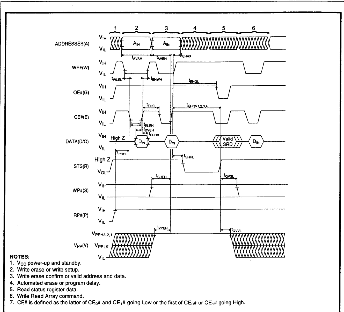
Figure 20. AC Waveform for CE#-Controlled Write Operations
