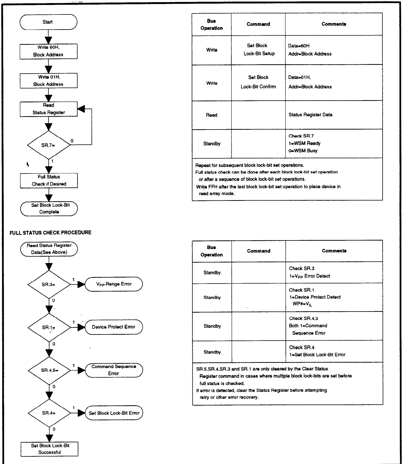
Figure 12. Set Block Lock-Bit Flowchart
