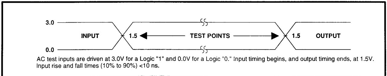
Figure 16. Transient Input/Output Reference Waveform for V_{CC}=5V\pm 0.5V (Standard Testing Configuration)
