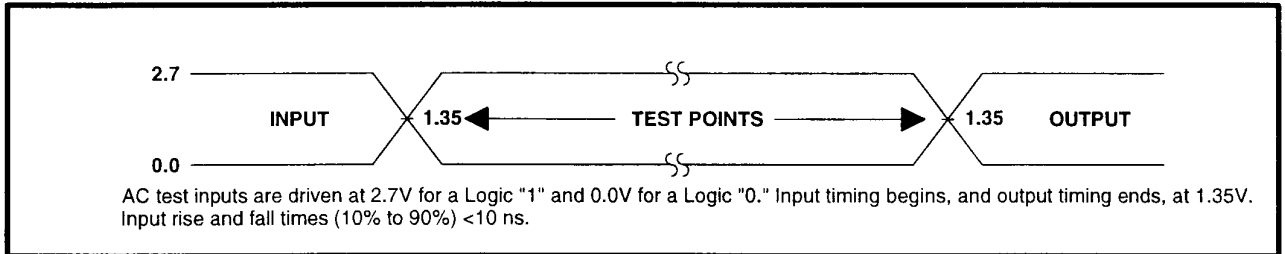
Figure 14. Transient Input/Output Reference Waveform for V_{CC}=2.7V-3.6V
