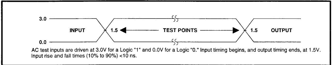
Figure 15. Transient Input/Output Reference Waveform for V_{CC}=3.3V\pm 0.3V and V_{CC}=5V\pm 0.25V (High Speed Testing Configuration)
