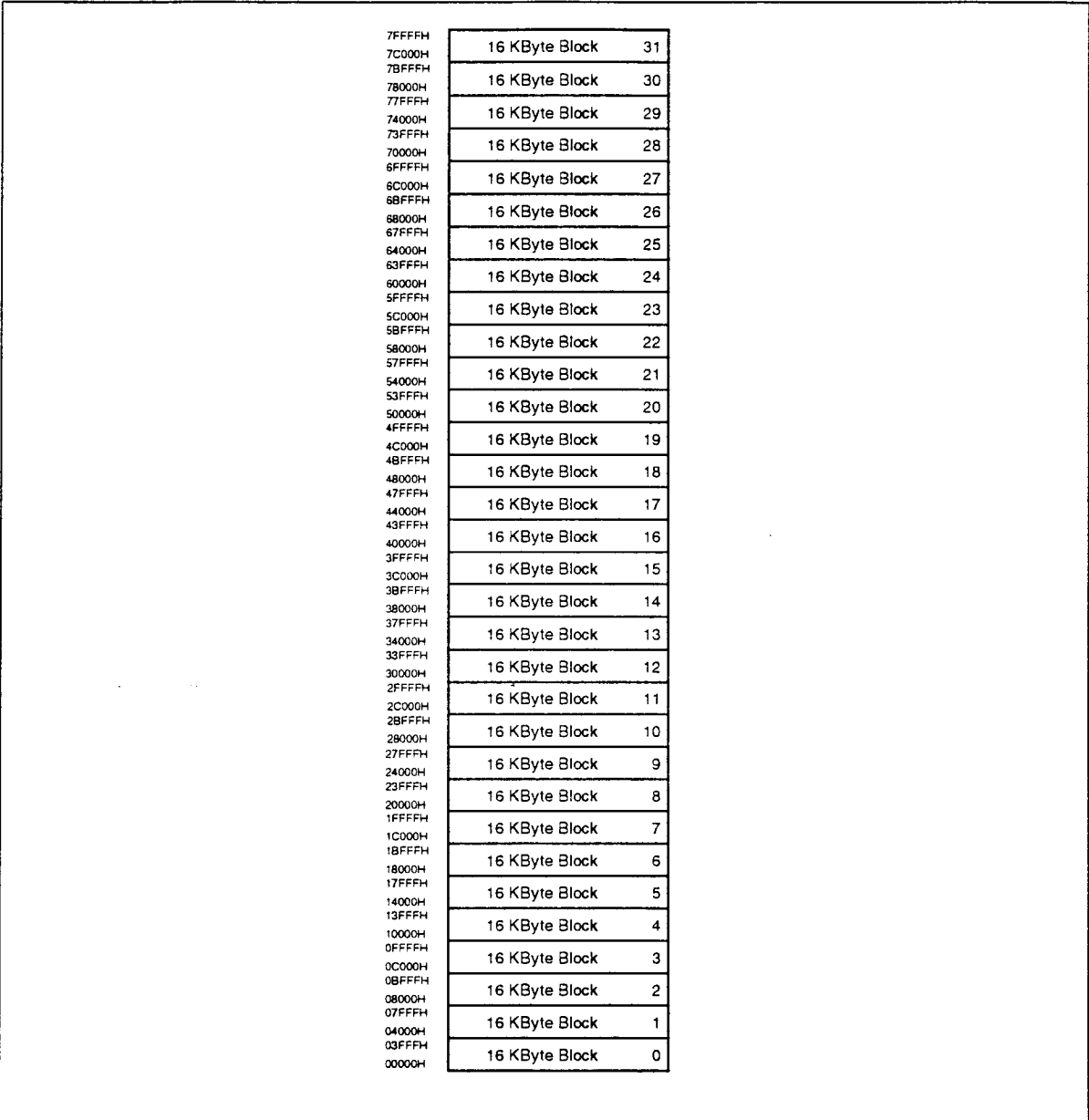
Figure 3. LH28F400SUHE-NC80 Memory Map (Byte-wide mode)
