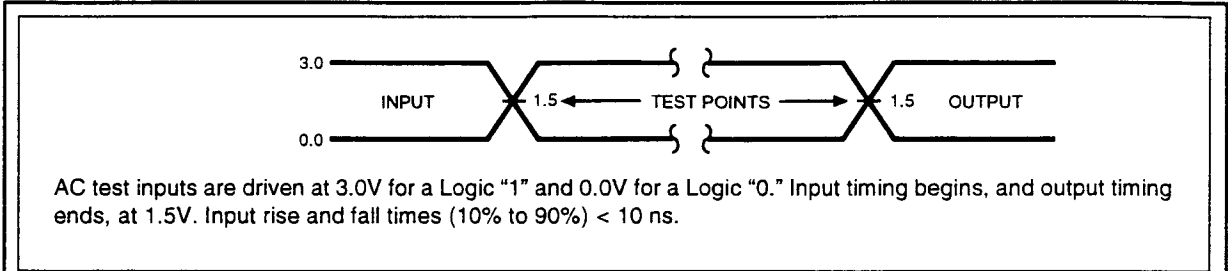
Figure 4. Transient Input/Output Reference Waveform ( V_{cc} = 5.0V )
