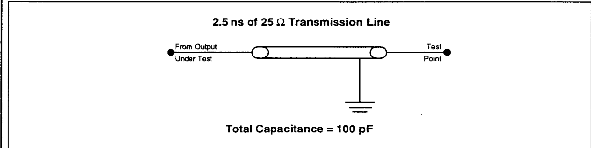
Figure 5. Transient Equivalent Testing Load Circuit ( V_{cc} = 5.0V )
