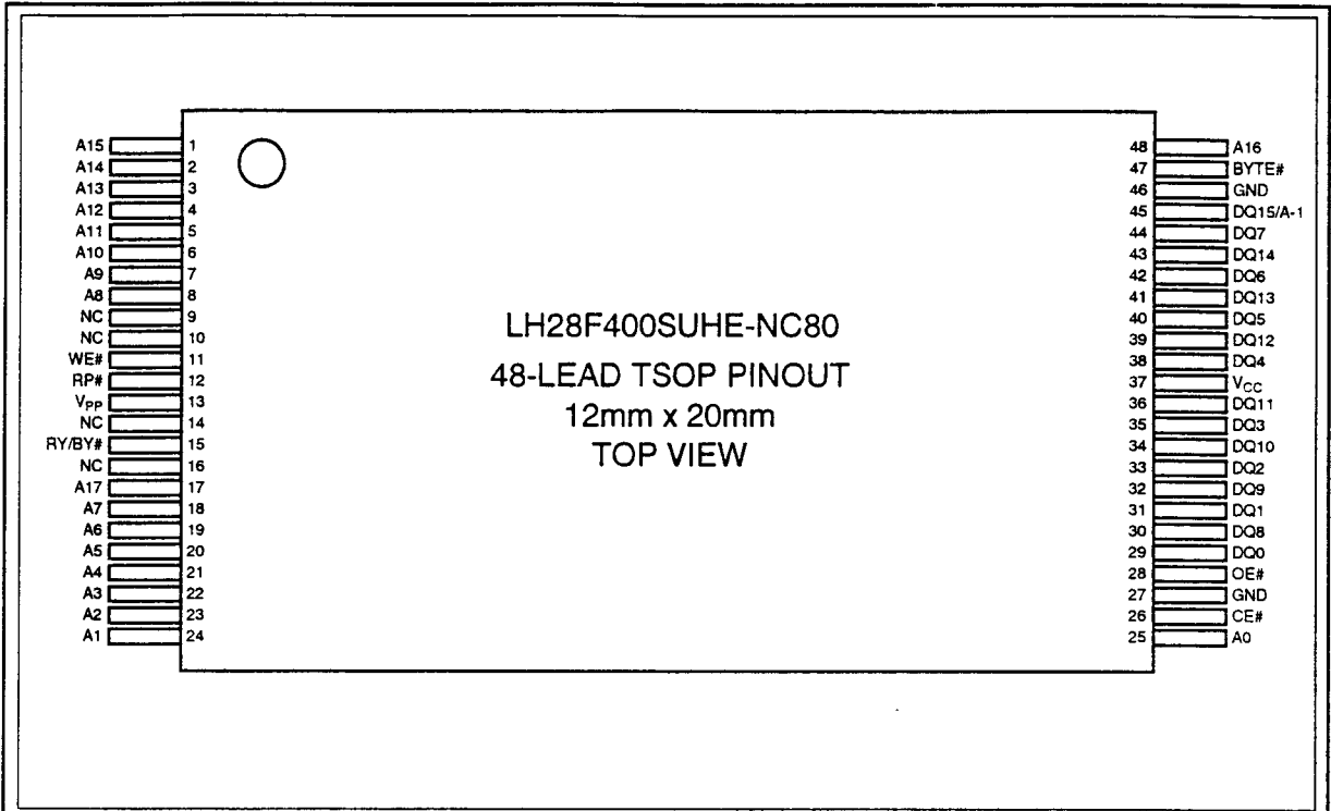
Figure 2. TSOP Configuration
