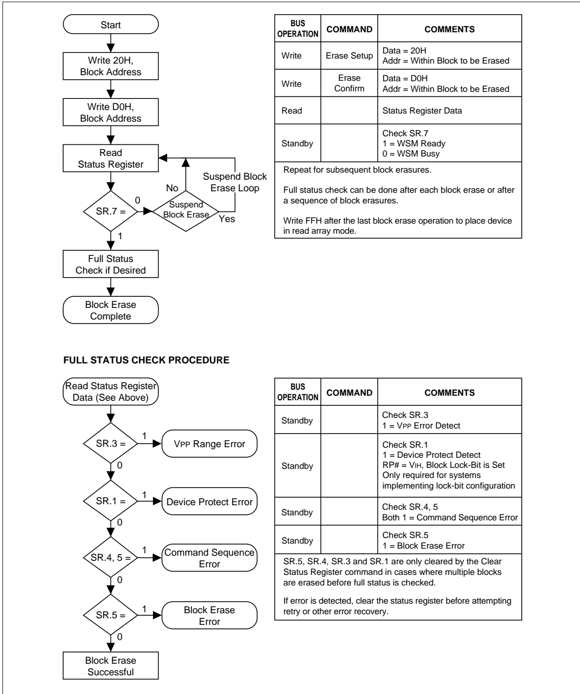
Fig. 3 Automated Block Erase Flowchart
