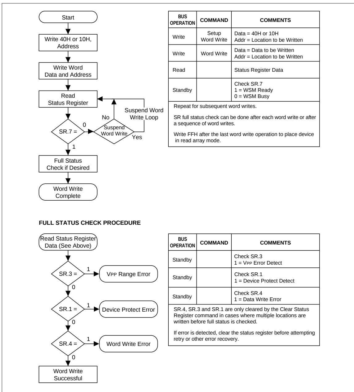
Fig. 4 Automated Word Write Flowchart
