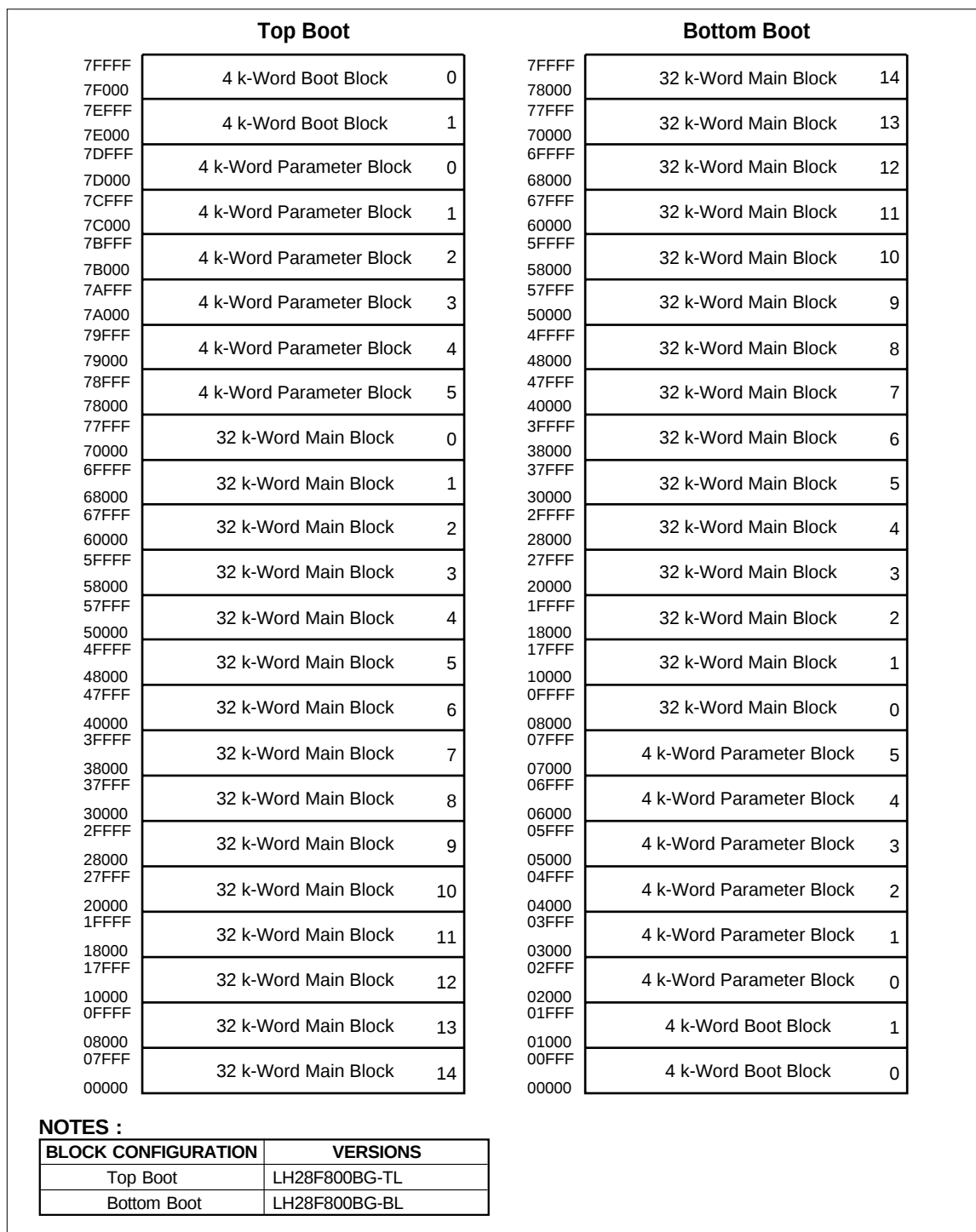
Fig. 1 Memory Map
