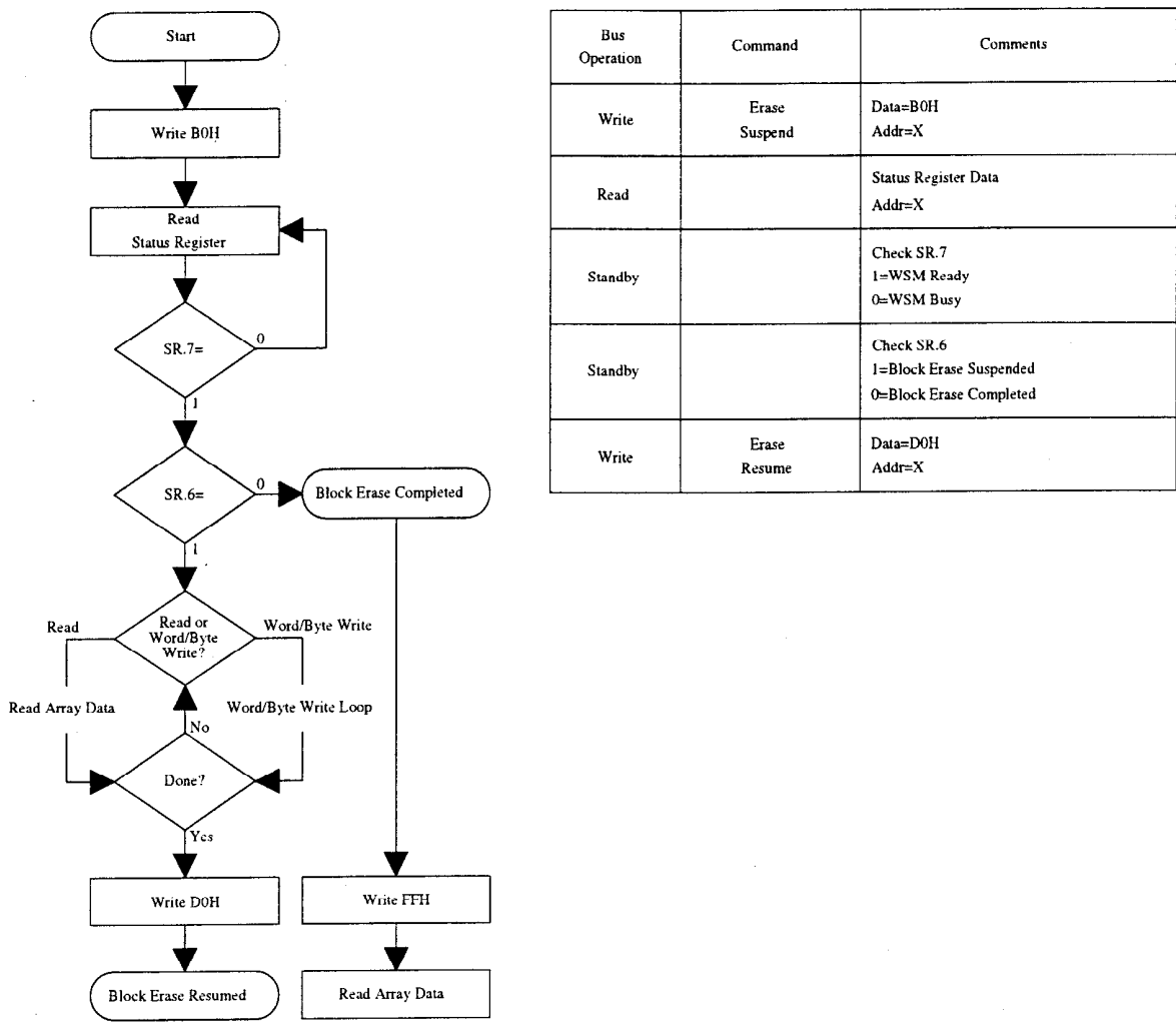
Figure 7. Block Erase Suspend/Resume Flowchart
