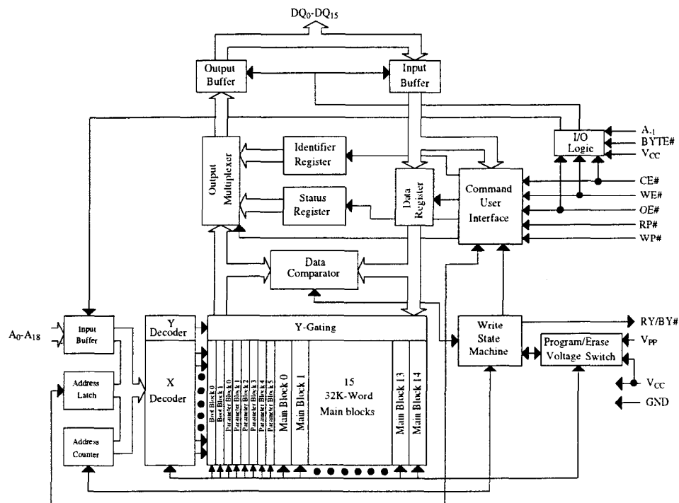
Figure 1. Block Diagram
