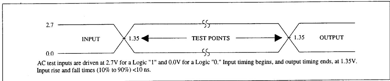
Figure 9. Transient Input/Output Reference Waveform for V_{CC}=2.7V-3.6V
