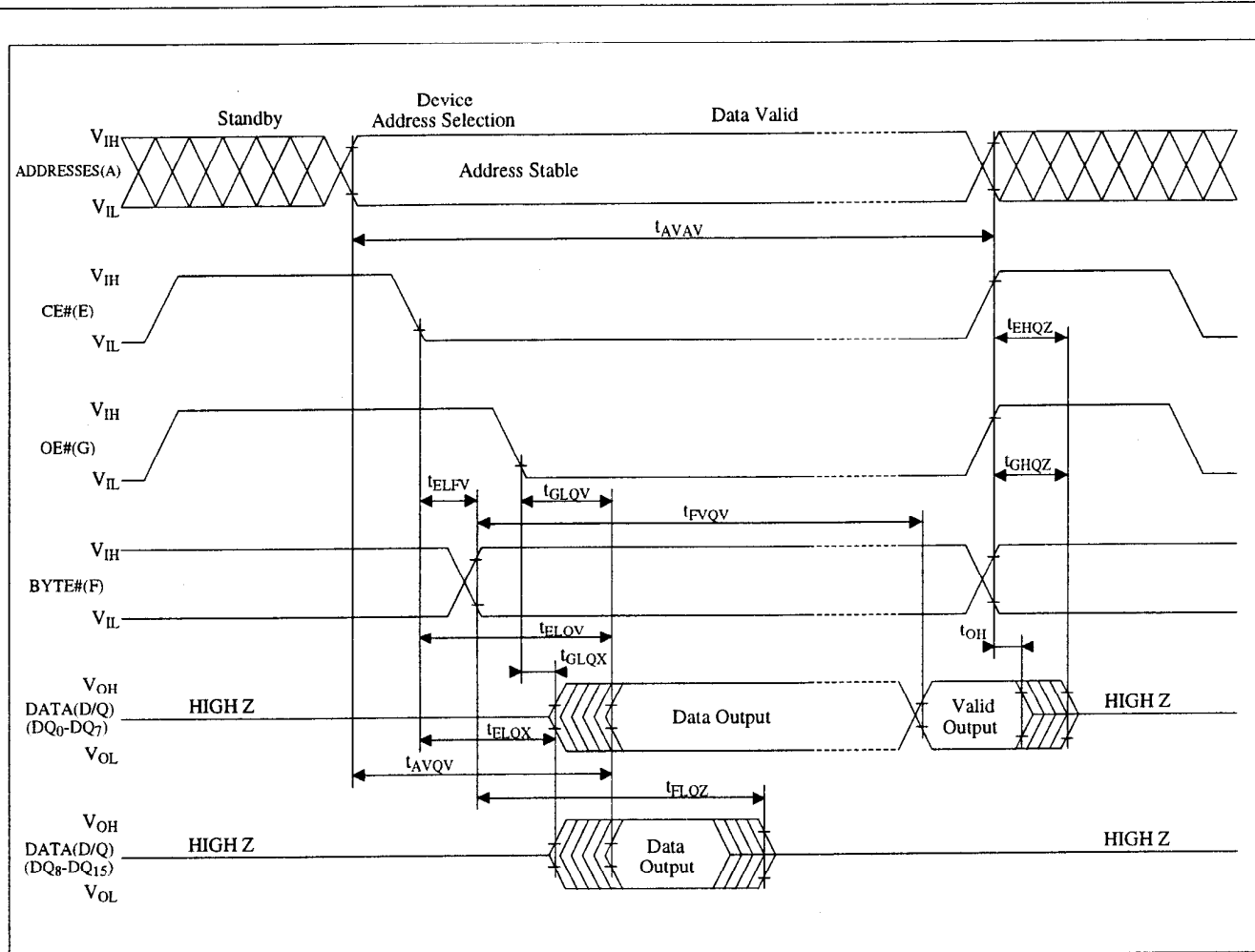
Figure 12. BYTE# timing Waveform
