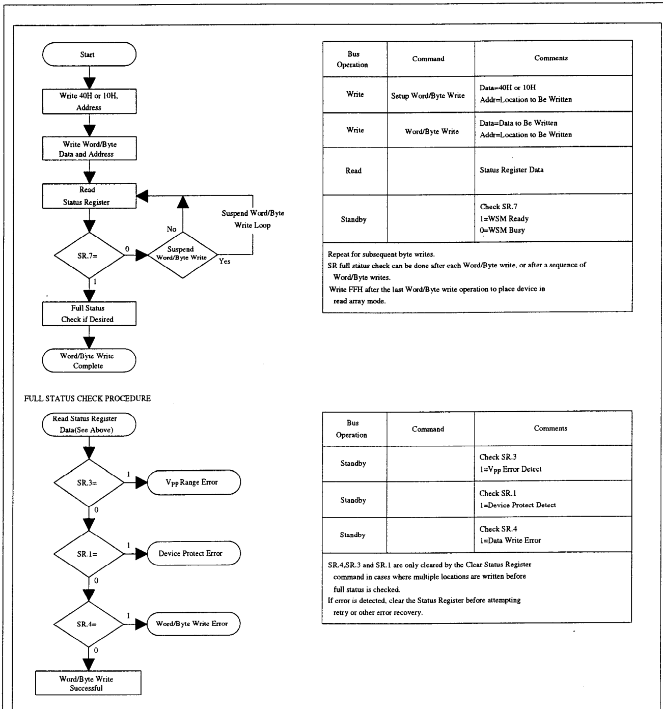
Figure 6. Automated Word/Byte Write Flowchart
