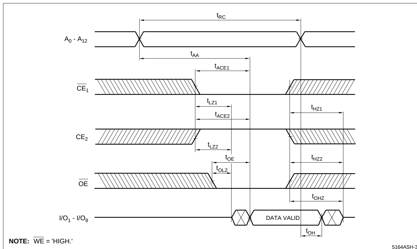
Figure 5. Read Cycle
