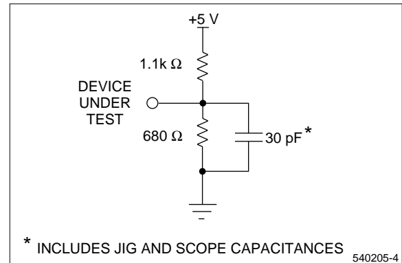
Figure 8. Output Load Circuit
