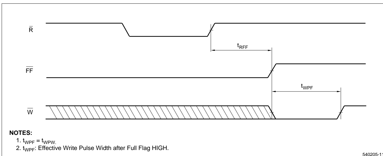
Figure 16. Full Flag Timing
