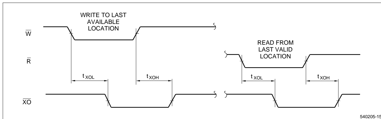
Figure 19. Expansion-Out Timing
