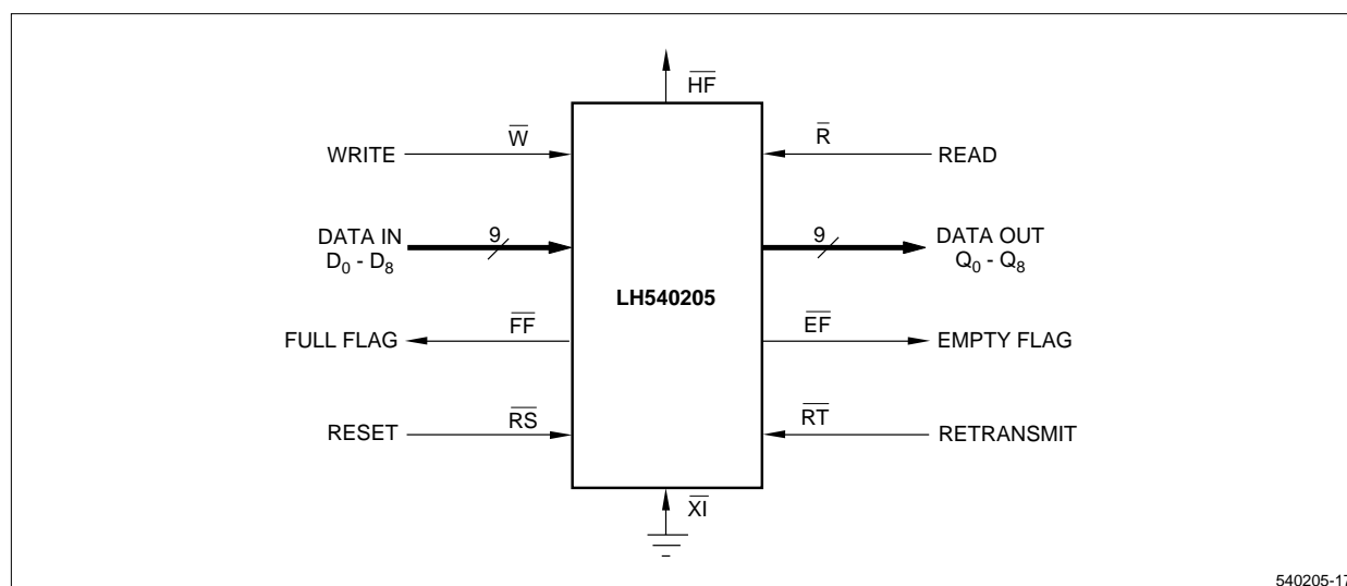
Figure 3. Standalone FIFO (8192 × 9)
