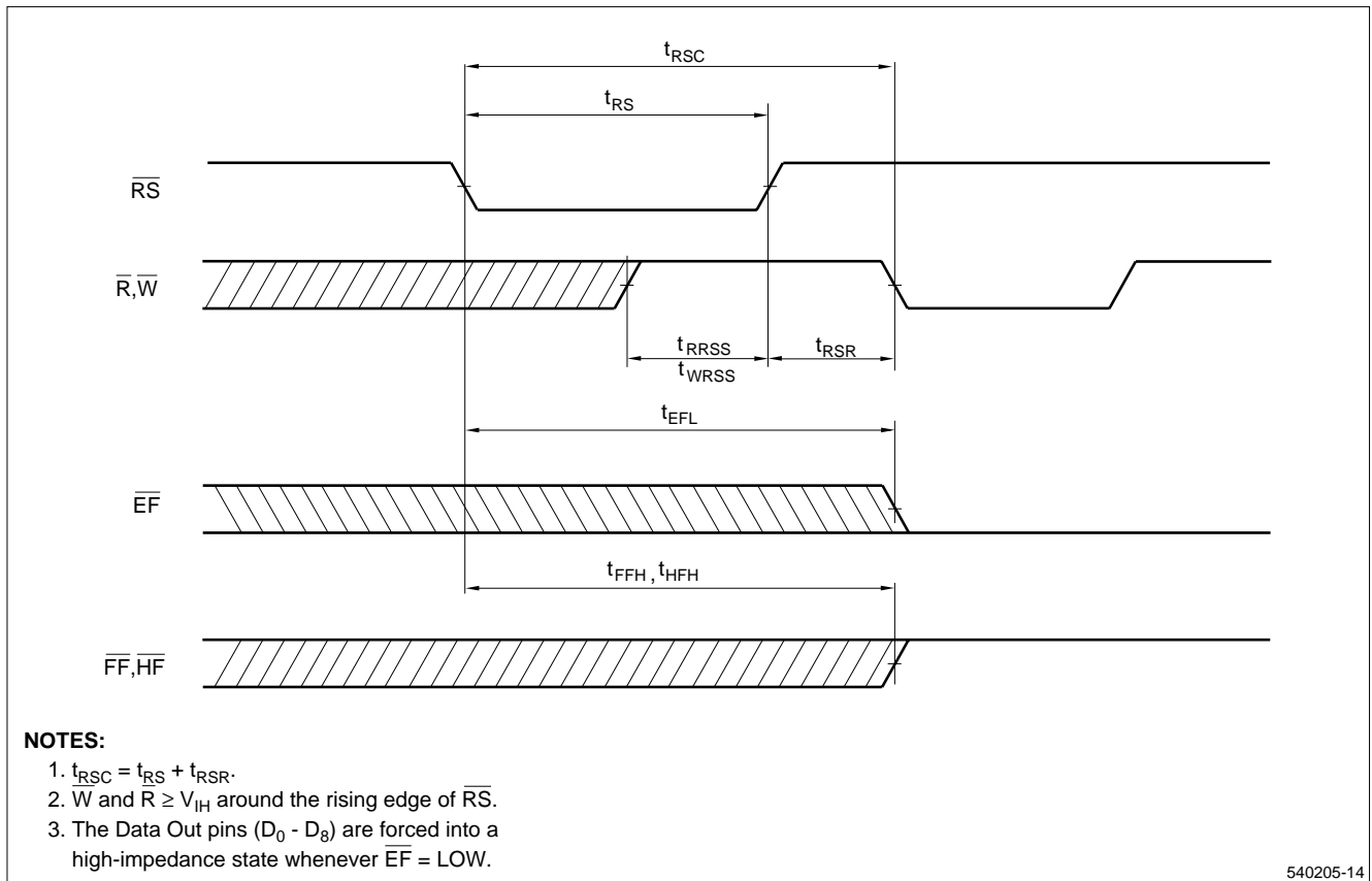
Figure 9. Reset Timing
