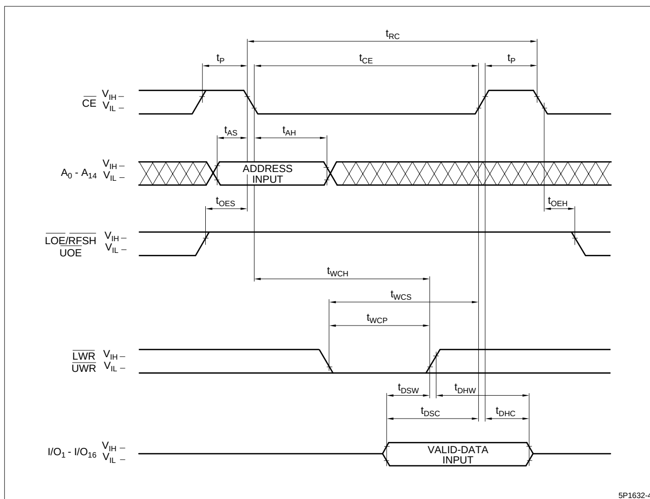
Figure 5. Write Cycle
