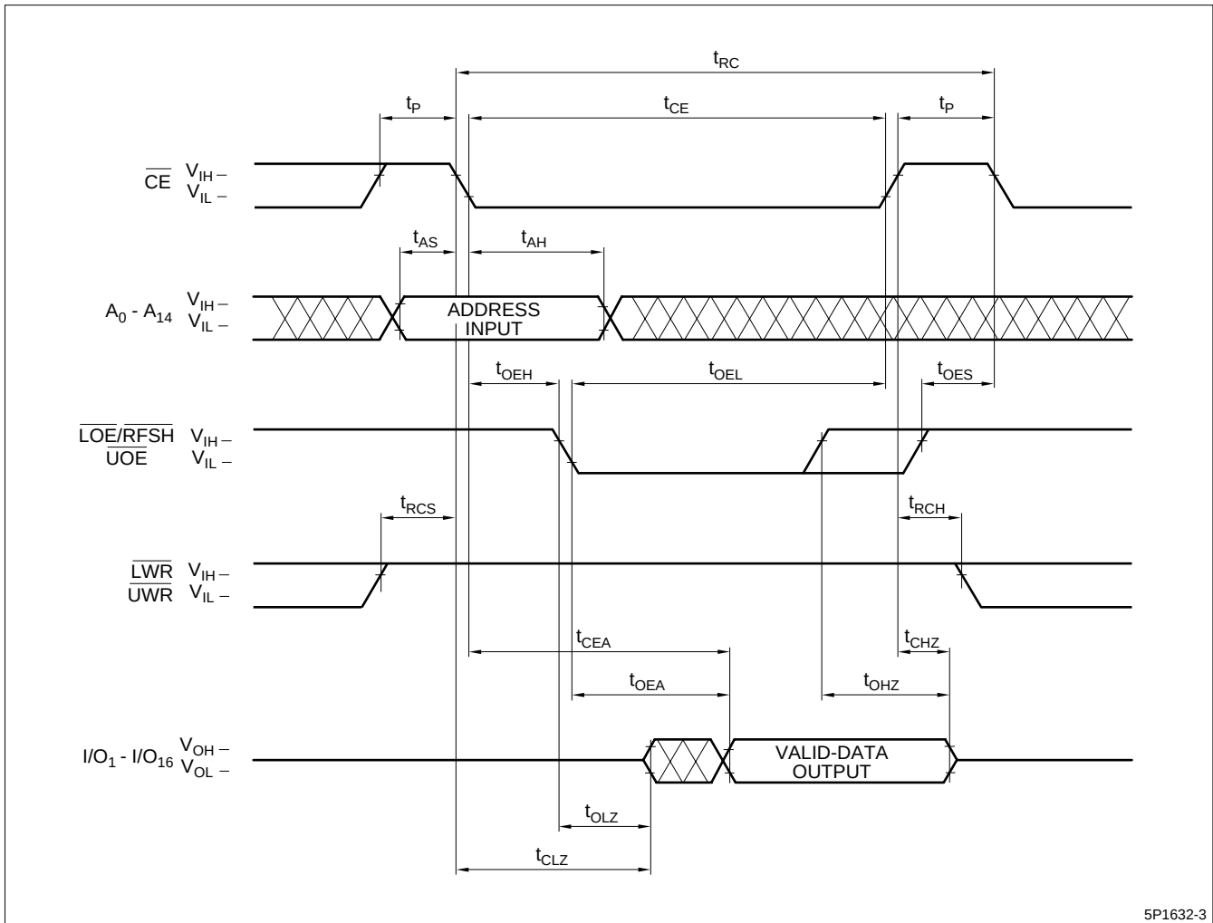
Figure 4. Read Cycle
