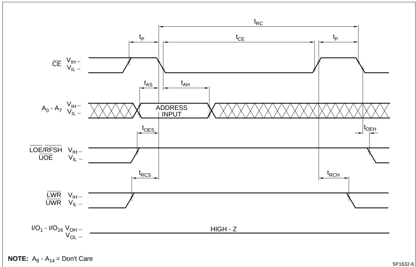
Figure 7. \overline{CE} Only Refresh Cycle
