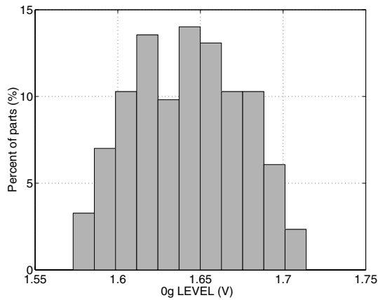
Figure 5. x-axis 0-g level at 3.3V
