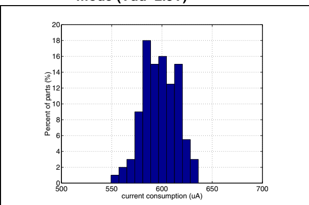
Figure 25. Current consumption in Operational mode (Vdd=2.5V)
