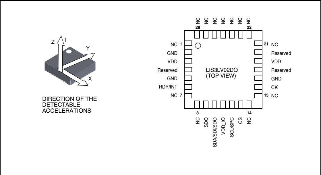
Figure 2. Pin Connection
