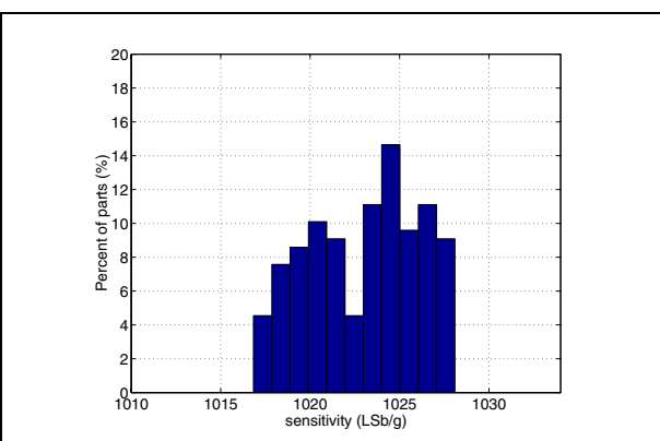
Figure 15. z-axis sensitivity at 2.5V
