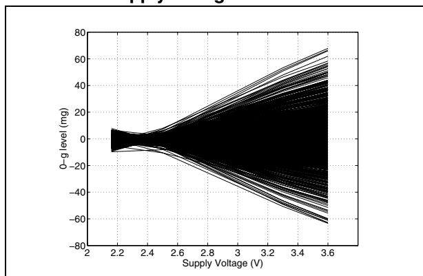
Figure 22. x and y axis 0-g level as function of supply voltage
