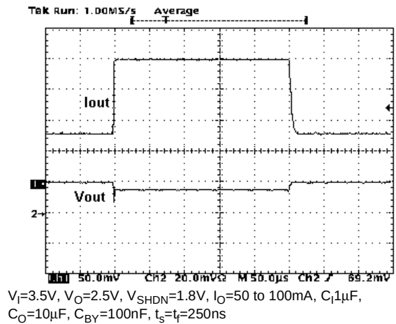
Figure 28 : Load Transient
