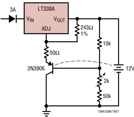
Temperature Compensated Lead Acid Battery Charger
