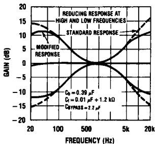
FIGURE 6. Tone Characteristic (Gain vs Frequency) TL/H/5142-9
