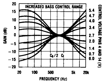
FIGURE 5. Tone Characteristic (Gain vs Frequency) TL/H/5142-8
