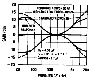
FIGURE 6. Tone Characteristic (Gain vs Frequency)
