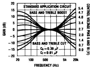
FIGURE 1. Tone Characteristic (Gain vs Frequency)
