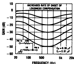
FIGURE 12. Loudness Compensated Volume Characteristic
