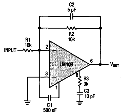
Feedforward Compensation
