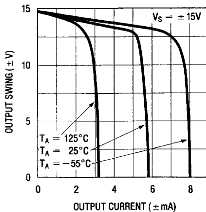
Output Swing
