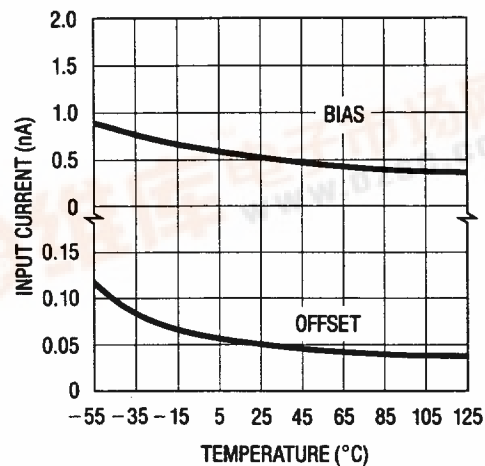
Input Currents
