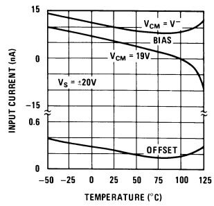
Input Current
