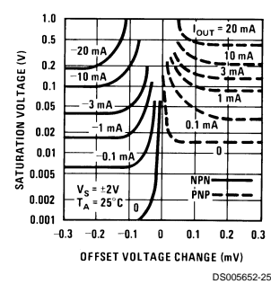
Output Saturation Characteristics
