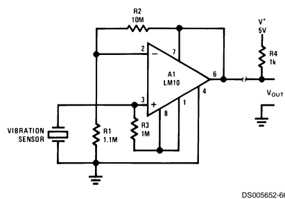
Remote Amplifier
