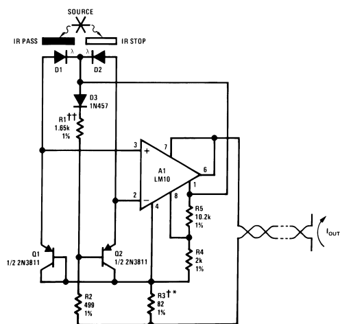
Optical Pyrometer
