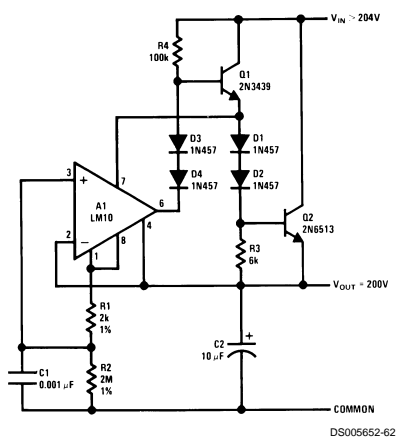
HV Regulator
