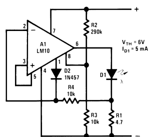
Battery-threshold Indicator
