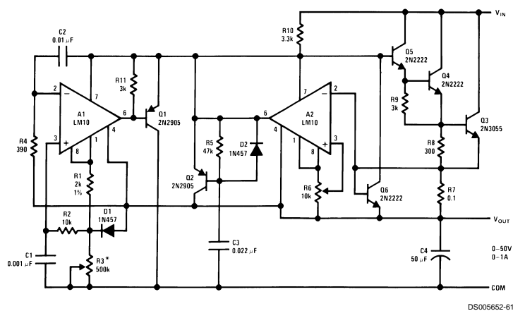
Laboratory Power Supply
