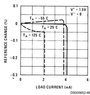
Load Regulation
