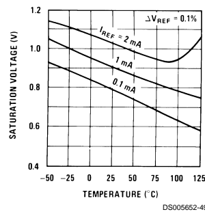
Output Saturation
