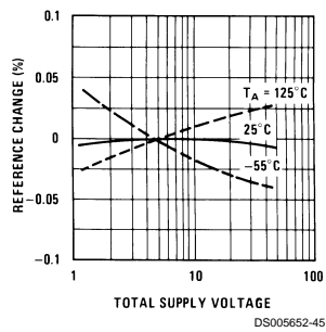
Line Regulation
