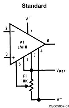
Op Amp Offset Adjustment
