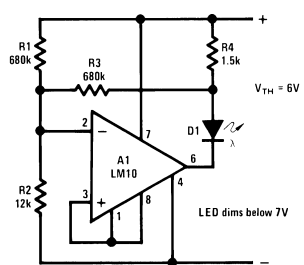
Battery-level Indicator
