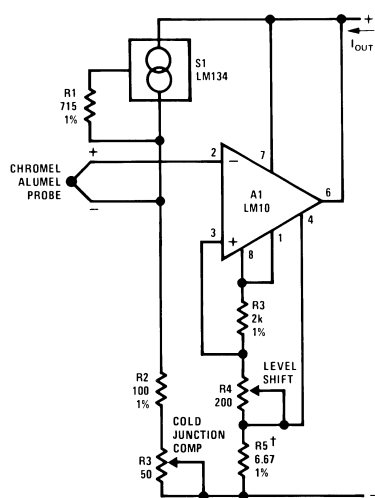
Thermocouple Transmitter
