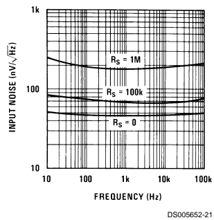
Input Noise Voltage
