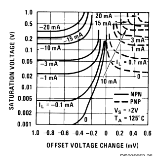
Output Saturation Characteristics
