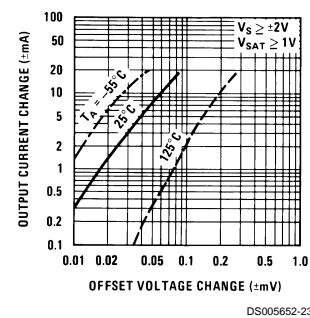
Transconductance
