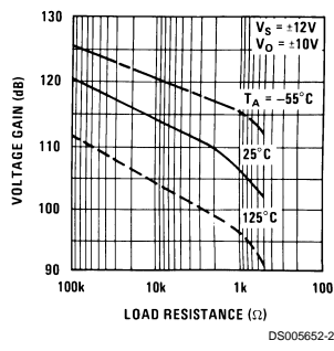
DC Voltage Gain
