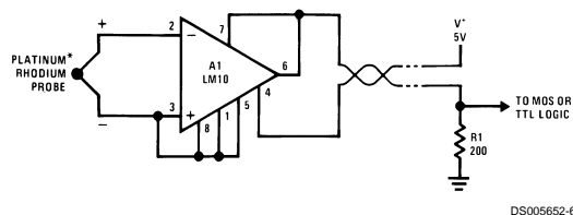
Flame Detector
