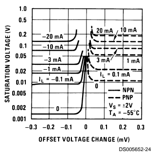
Output Saturation Characteristics
