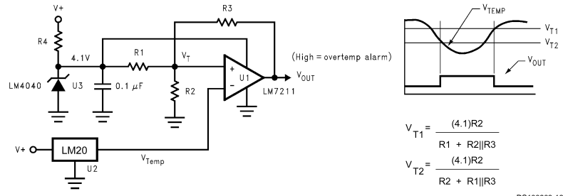
FIGURE 6. Centigrade Thermostat
