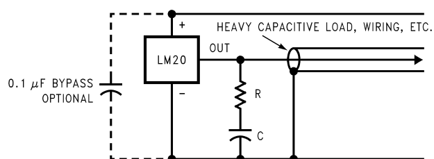
FIGURE 5. LM20EP with Filter for Noisy Environment and Capacitive Loading greater than 300 pF. Either placement of resistor as shown above is just as effective.
