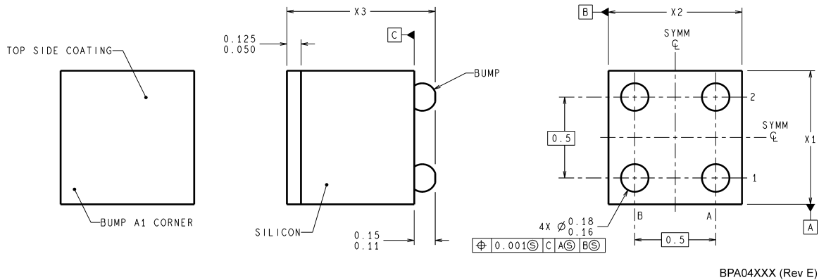
4-Bump micro SMD Ball Grid Array Package (Small Bump) NS Package Number BPA04DDC The following dimensions apply to the BPA04DDC package shown above: X1=X2 = 853µm ±30µm, X3= 900µm ±50µm
