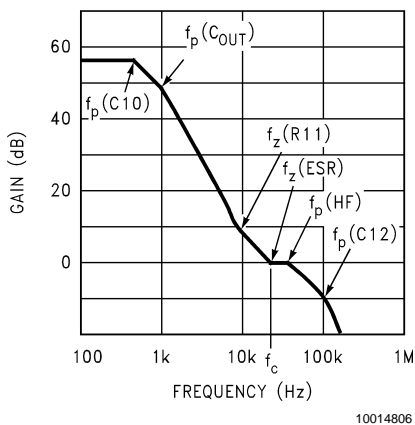
FIGURE 5. Typical Loop Gain Plot
