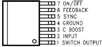
TO-263 Package Top View
