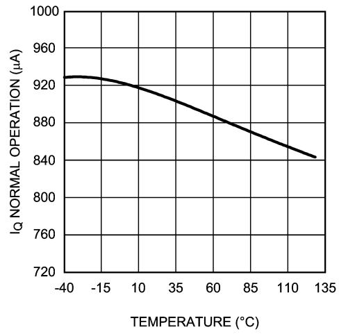
I_Q vs Temperature (Normal Operation)
