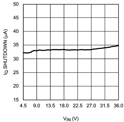
I_Q vs V_{IN} (Shutdown)
