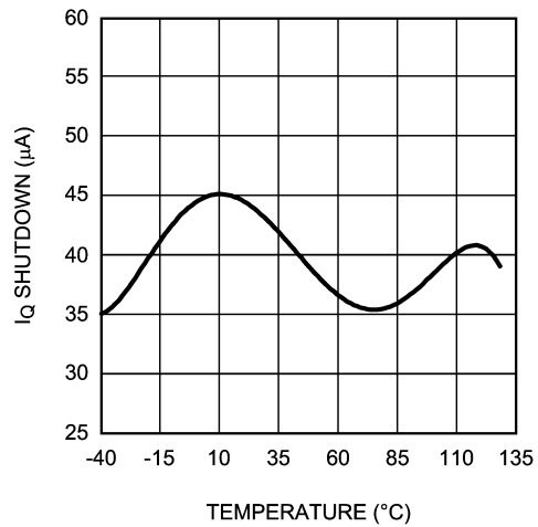
I_Q vs Temperature (Shutdown)
