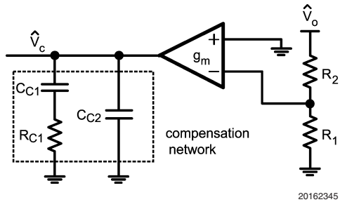
FIGURE 8. Compensation Network
