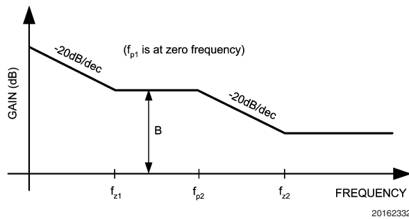
FIGURE 7. Output-Control Transfer Function
